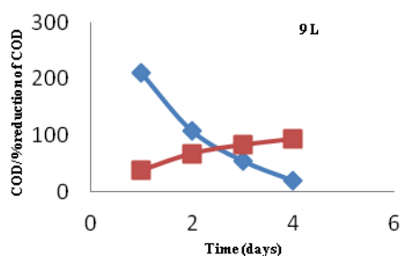
Fig 13: COD % reduction of COD on Time for 9 L volume electrolyte
