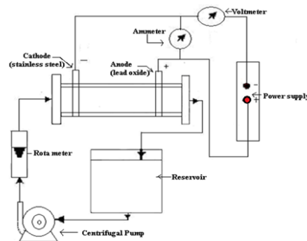
Fig.1: Schematic representation of Electrochemical Oxidation System
