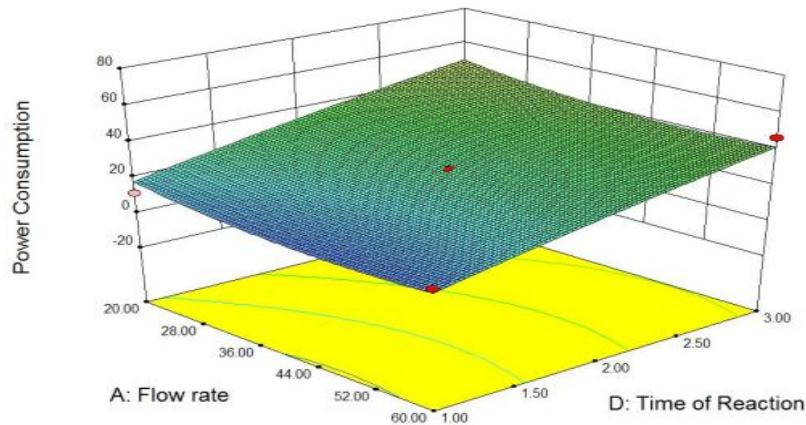
Fig 8: Flow rate and Time on Power consumption
